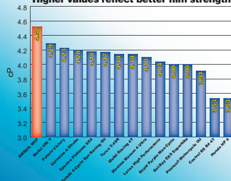
10W-40 Motorcycle Oil High-Temperature Viscosity Protection ASTM D-4683 Test Date August 2008 Higher values reflect better film strength.
